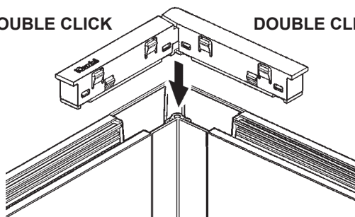
art. PB42 Superrail track: Up/down
